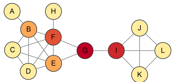
Figure 18: Analysis of a simple network using different centrality measurements. Nodes are colored according to each metric using a yellow-to-red gradient (yellow: lowest value, red: highest value). Network visualization and analysis were performed in Cytoscape.
