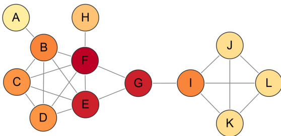
Figure 18: Analysis of a simple network using different centrality measurements. Nodes are colored according to each metric using a yellow-to-red gradient (yellow: lowest value, red: highest value). Network visualization and analysis were performed in Cytoscape.
