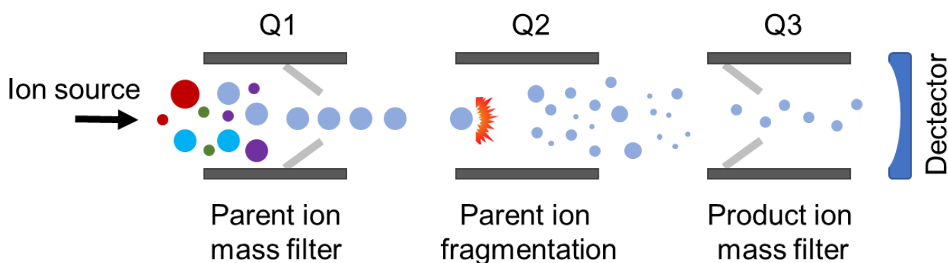
Figure 9: Schematic diagram of typical QqQ system. Three quadrupoles enable precursor selection, fragmentation, and the fragment ion selection.
