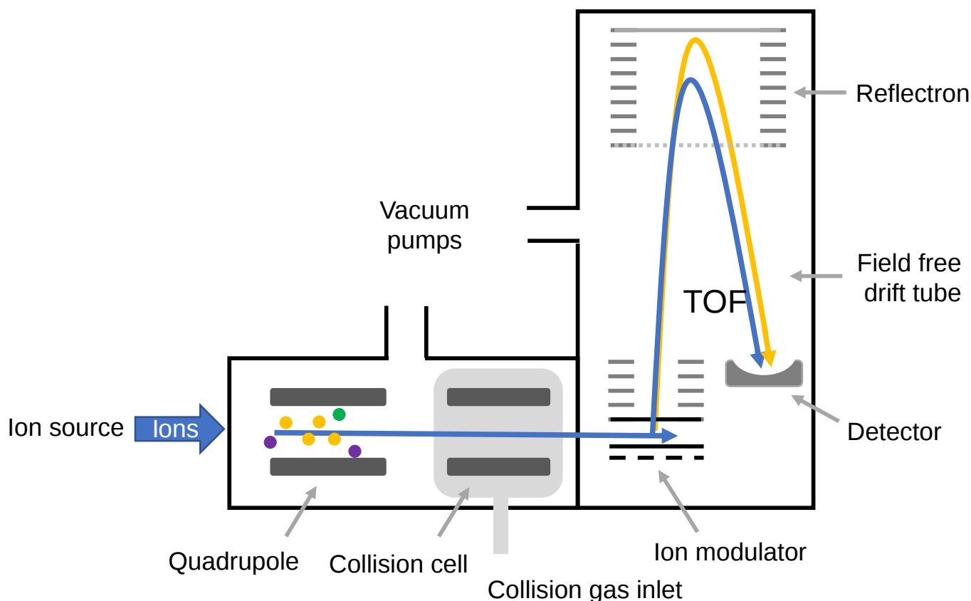
Figure 10: Schematic diagram of a typical quadrupole time-of-flight mass spectrometer. Like a QQQ, a Q-TOF will have two quadrupoles for selection and fragmentation followed by the TOF for the final higher resolution separation and detection.
