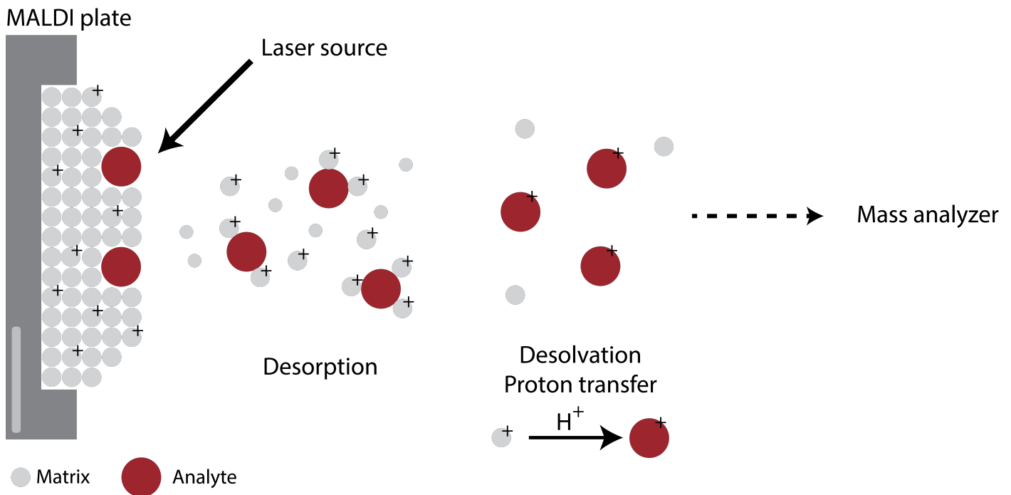
Figure 6: MALDI The analyte-matrix mixture is irradiated by a laser source, leading to ablation. Desorption and proton transfer ionize the analyte molecules that can then be accelerated into a mass spectrometer.
