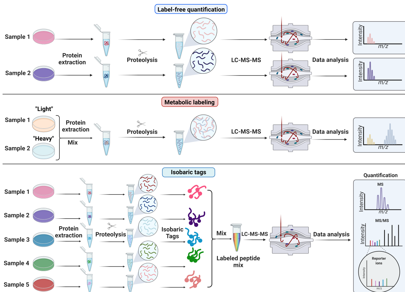
Figure 3: Quantitative strategies commonly used in proteomics. A few non-comprehensive examples of quantification methods are shown. A) Label-free quantification. Proteins are extracted from samples, enzymatically hydrolyzed into peptides and analyzed by mass spectrometry. Extracted ion chromatograms from peptides are compared across samples that are analyzed sequentially. B) Metabolic labelling. Stable isotope labeling by amino acids in cell culture (SILAC) is based on feeding cells stable isotope labeled amino acids ("light" or "heavy"). Samples grown with heavy or light amino acids are mixed before cell lysis. The relative intensities of the heavy and light peptide are used to compute protein differences between samples. C) Isobaric or chemical labelling. Proteins are isolated separately from samples, enzymatically hydrolyzed into peptides, and then chemically tagged with isobaric stable isotope labels. These isobaric tags produce unique reporter mass-to-charge ( m/z ) signals that are produced upon fragmentation with
